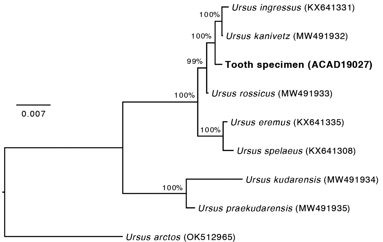
Text-fig. 2. Phylogenetic position of anomalous tooth of U. kanivetz from Pobeda Cave based on ancient mtDNA.
