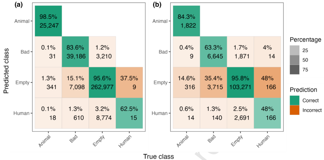
Figure 2. Confusion matrix for the results of the complete workflow applied to the test data, which represents a full season of data not used in model development at (a) Finnmark and (b) Yamal. False positive model results were aggregated in the “Animal” class. The percentage and number of images with correct (diagonal, green) and incorrectly predicted classes (off-diagonal) are displayed.
