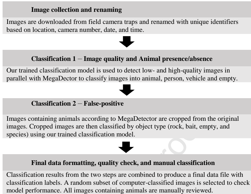
Figure 1. Time-lapse camera trap workflow. Data preparation and model steps are adapted from Böhner et al. (2022).
