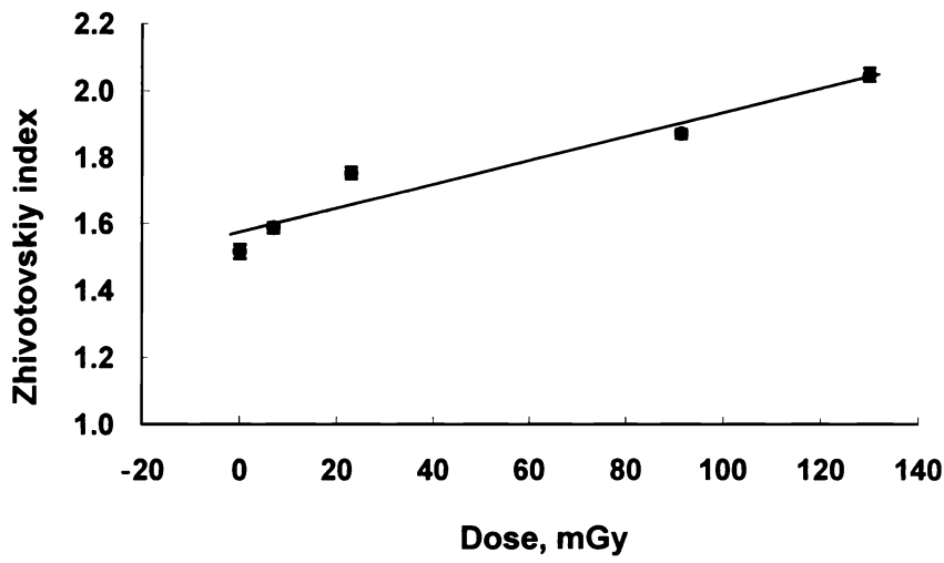
Figure 4. Phenotypic variability estimated via the Zhivotovskiy index (2005) in dependence on annual dose absorbed by generative organs of pine trees
