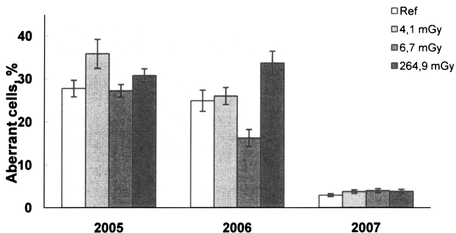
Figure 7. Aberrant cell frequency in root meristems of Scots pine seedlings after acute exposure of seeds to 15 Gy of \gamma -rays. * - difference from the Ref site is significant, p < 0.05 ; + - difference from the Ref1 site is significant, p < 0.05
