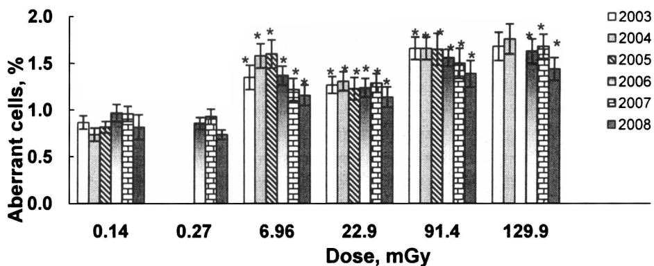
Figure 2. Aberrant cells in root meristem of germinated seeds (%) from Scots pine populations collected in the Bryansk Region of Russia, 2003-2008. Ref and Ref I are the reference populations. Significant difference from the reference populations: * - p < 0.05
