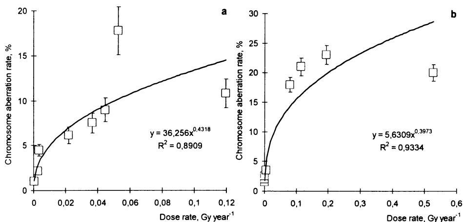
Figure 2. The dependence of chromosomal aberration rate from absorbed dose rate in cells of the common reed (a) and embryos of the gastopod pond snails (b) from water bodies within the Chernobyl exclusion zone.
