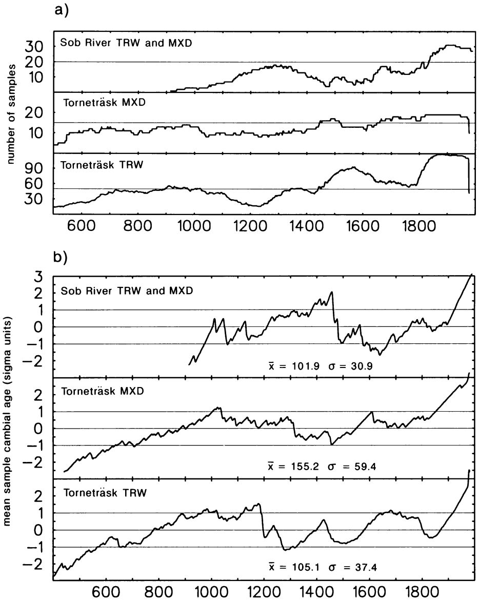
Figure 2: (a) Series replication in the Russian, Sob River and Swedish, Torneträsk ring-width (TRW) and maximum-latewood-density (MXD) chronologies (b) The cambial age of the same data averaged over all samples in each year. These data are plotted as standardized departures.
