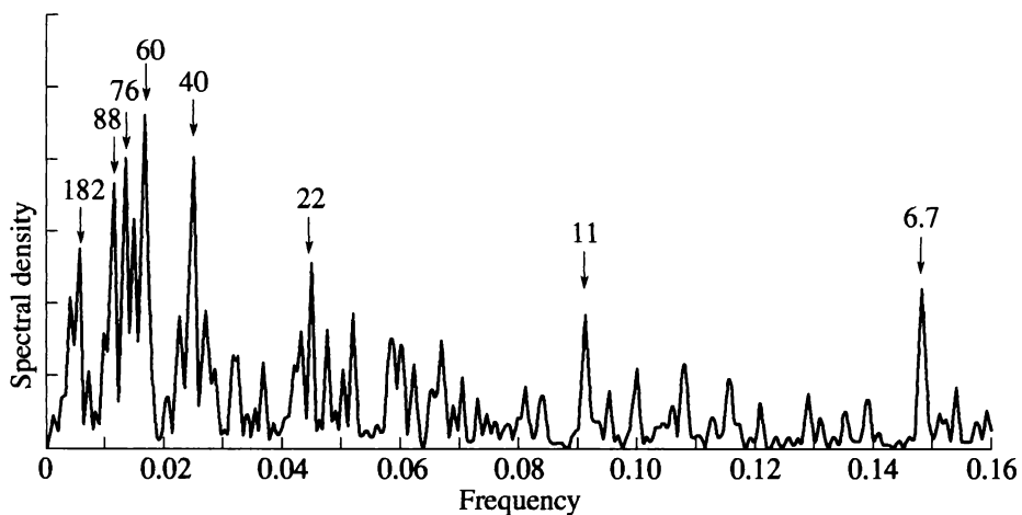
Fig. 4. The spectral density function for the generalized tree-ring chronology.
