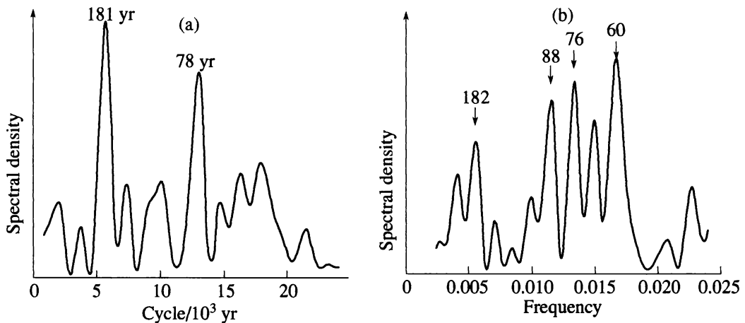
Fig. 3. (a) Fragments of spectral density function for oxygen isotope variations in the ice layers [5, 6] and (b) indices of tree growth.
