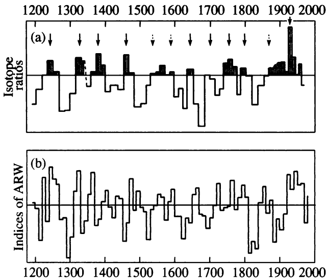
Fig. 2. (a) Comparison of the long-term temperature variations obtained from the analysis of the oxygen isotope ratios in the ice layers of Greenland [5, 6] and (b) the generalized ring-tree chronology for the Subarctic western and central Siberian sectors (the average over decades).
