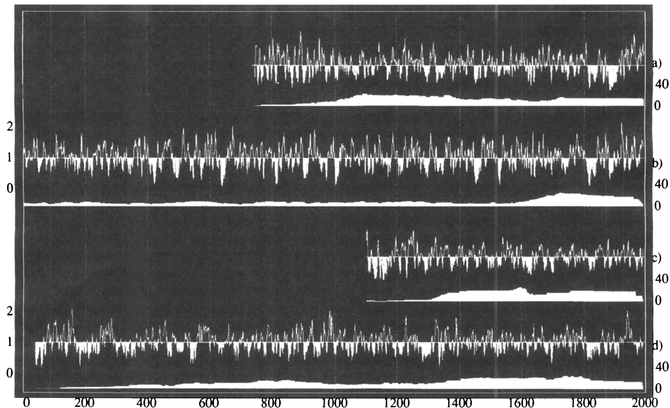
Fig. 1. The generalized tree-ring chronologies for larch (smoothed by the 5-yr moving-average): (a) Polar Urals, (b) southern Yamal, (c) Taz River, (d) eastern Taimyr. The diagram under each chronology (for a specified time interval) shows the number of tree specimens used for constructing the chronology. The left-hand abscissa shows the standardized growth indices, the right-hand abscissa indicates the number of specimens, and the ordinate shows calendar years.
